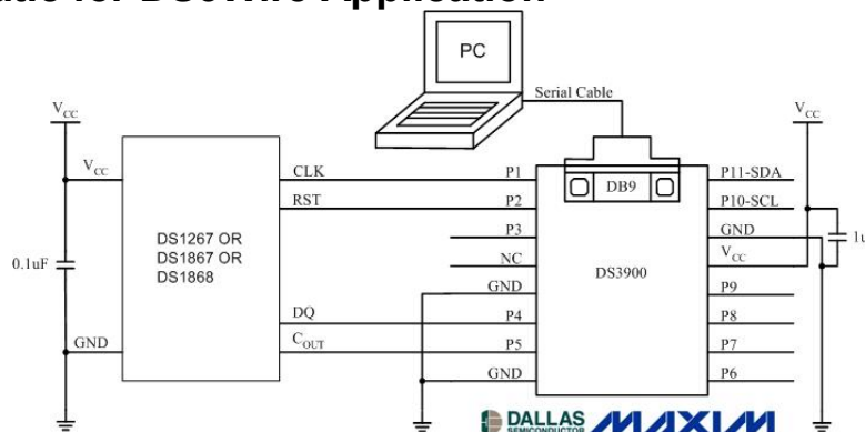
Figure 2. Schematic for DS3Wire Application
